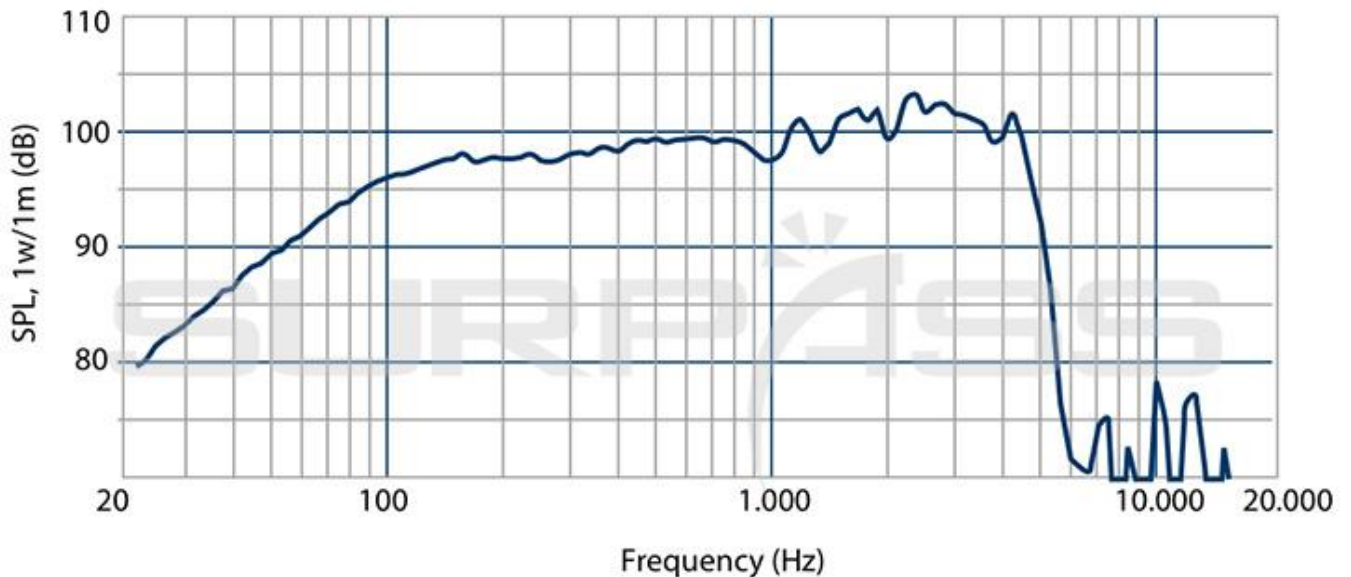
Sound Pressure Level/Mixer Frequency Sweeping Regulation
